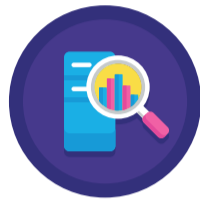
Data Science
