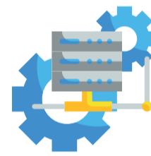
Computer systems
